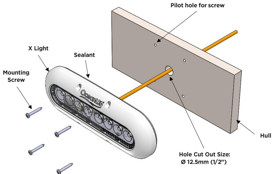
Exploded view of the standard assembly.
