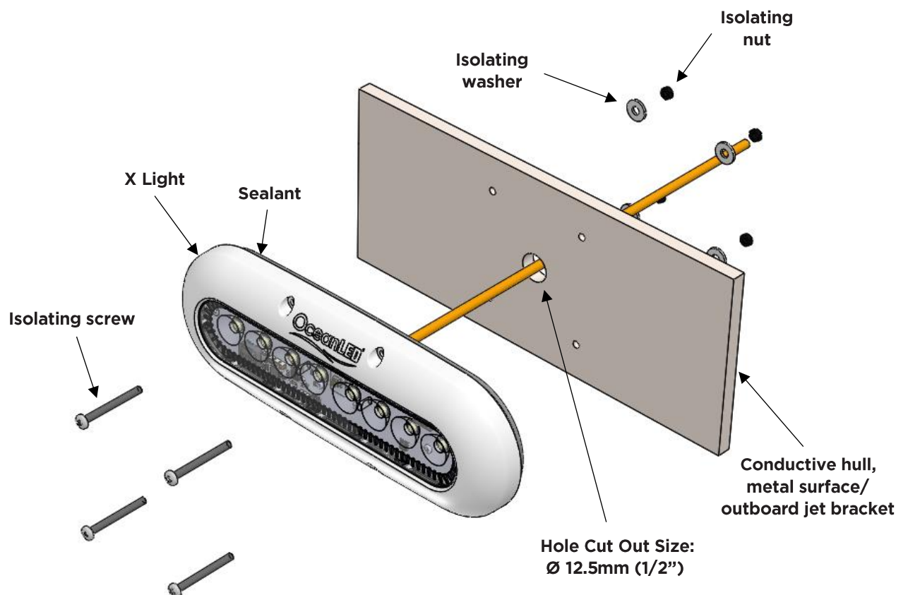
Exploded view of the assembly with Isolating Mounting Kit.
